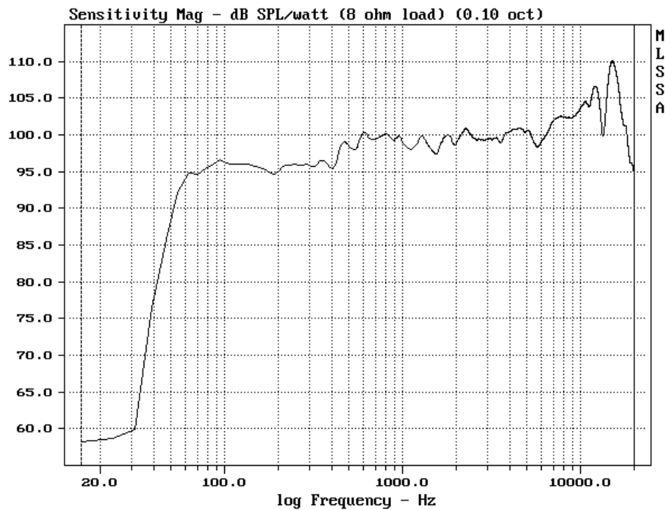
System 15-6 passiv Frequenzgang / Frequency Response
