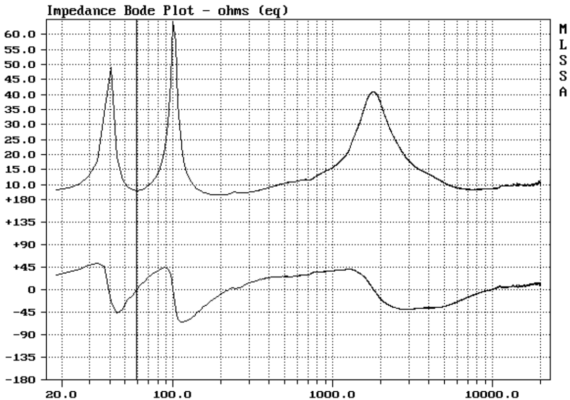
Impedance Response/Bode Plot GAE System 12TM (Fbox: 59Hz)
