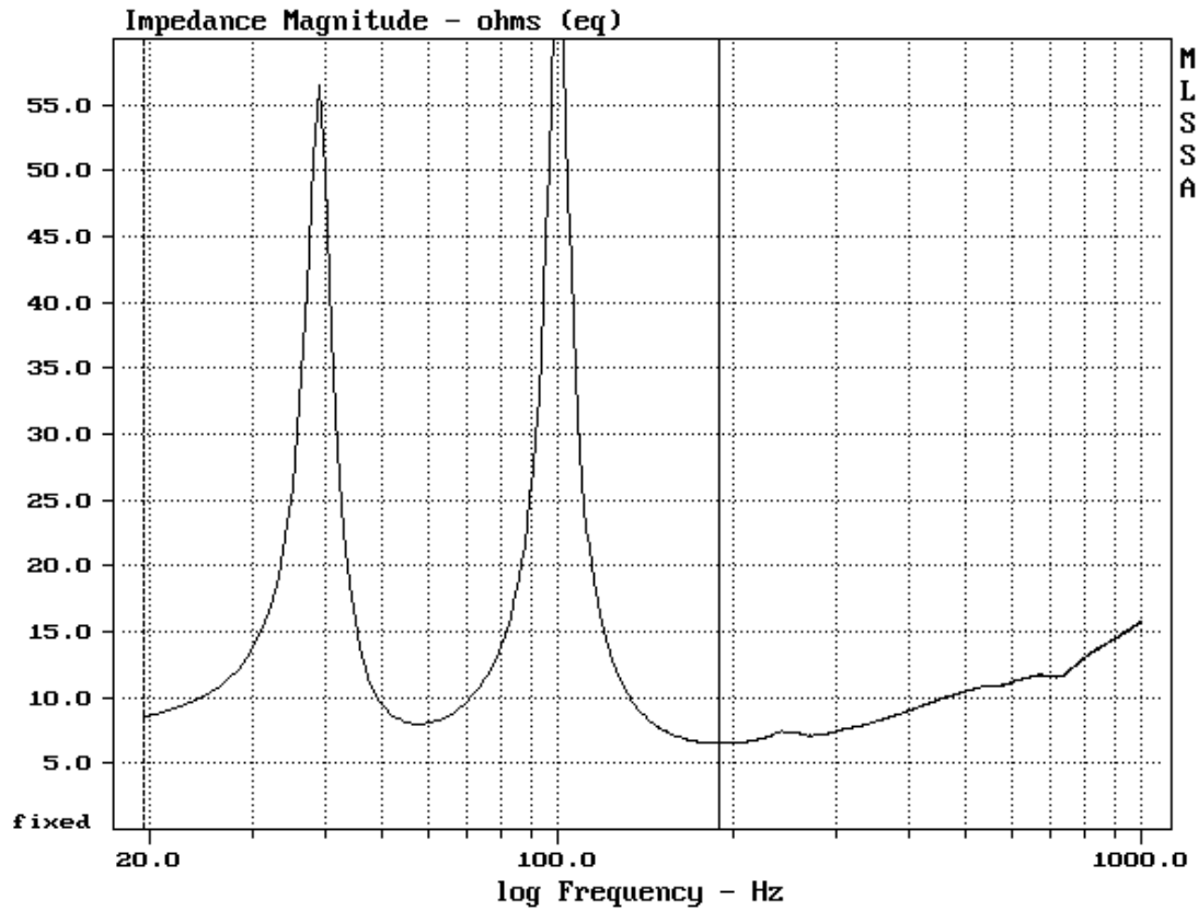
Impedance Response GAE System 12TM (Zmin 6,5 \Omega /190Hz)
