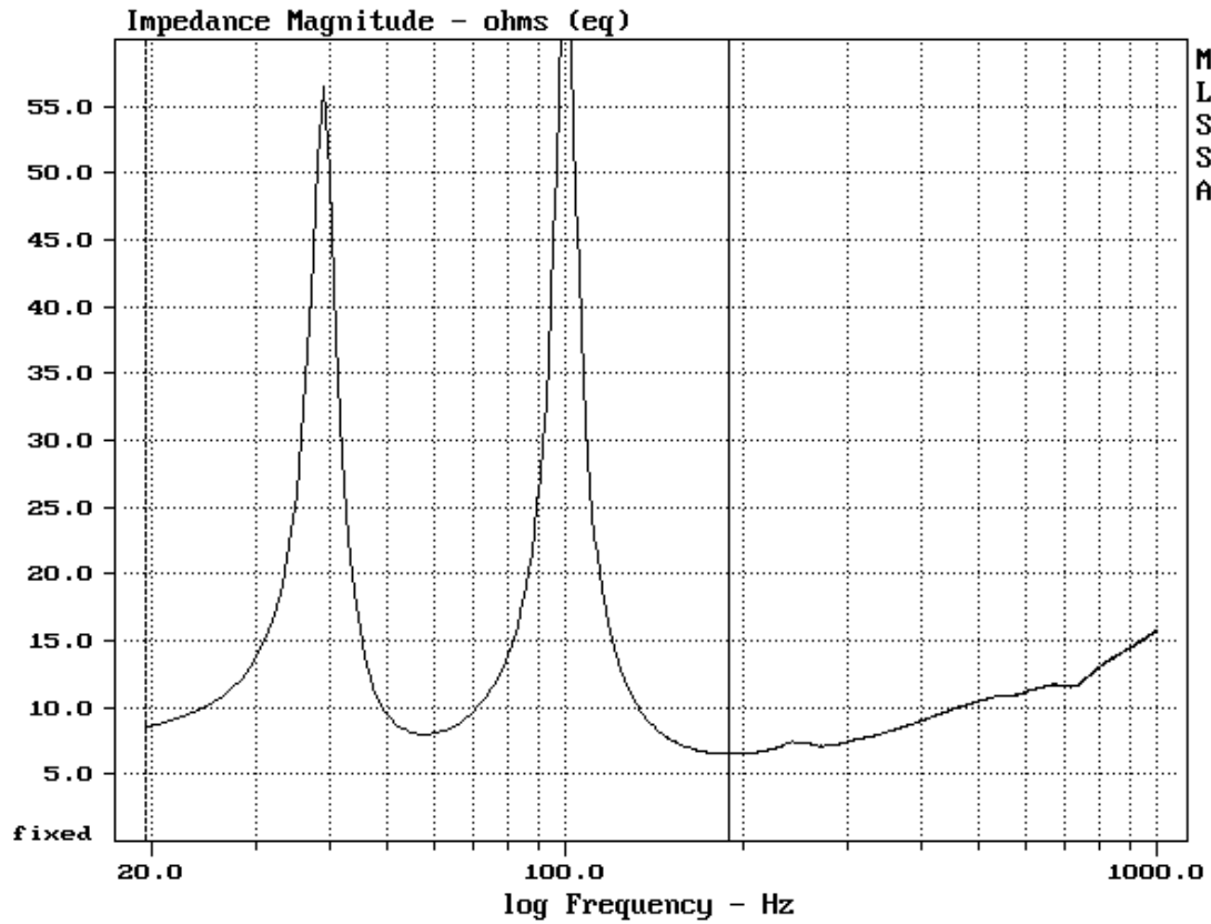
Impedance Response GAE System 12TM (Zmin 6,5Ω/190Hz)
