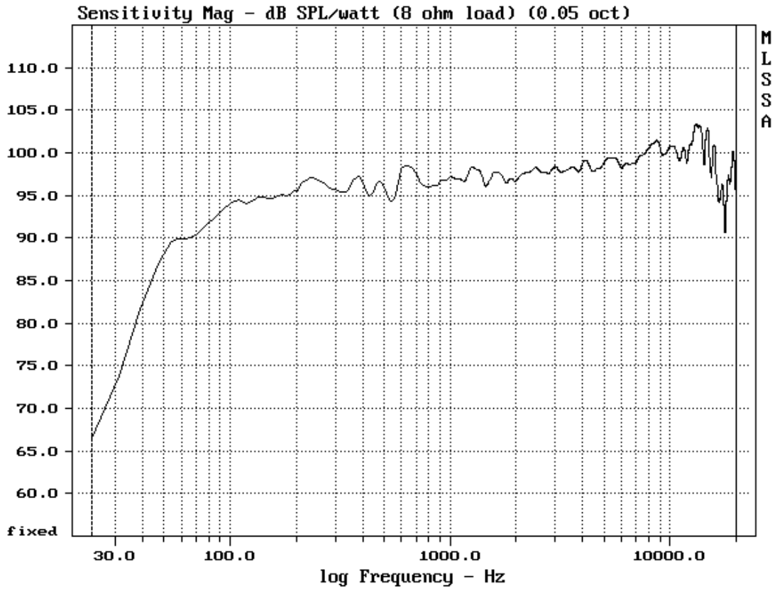
Frequency Response (Sensitivity) GAE System 12TM without controller
