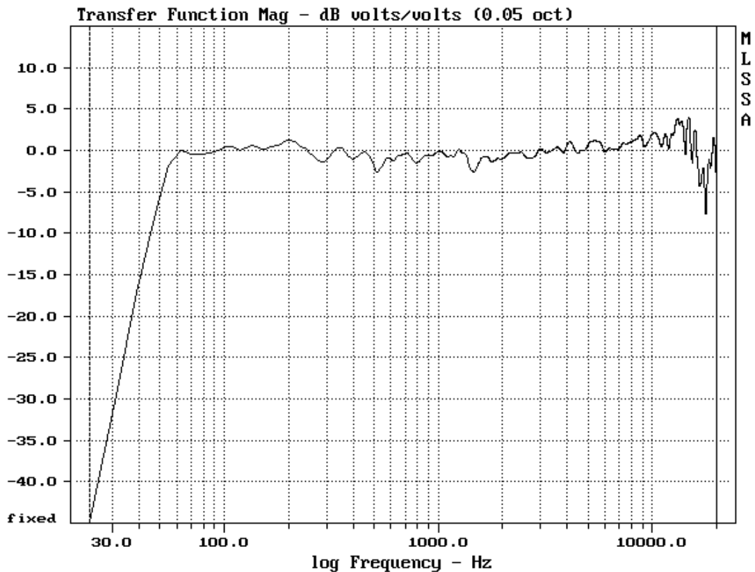
Frequency Response GAE System 12TM with controller
