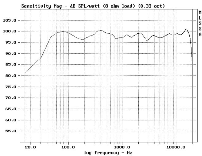
Frequency response GAE PS4475T - PS4475L
