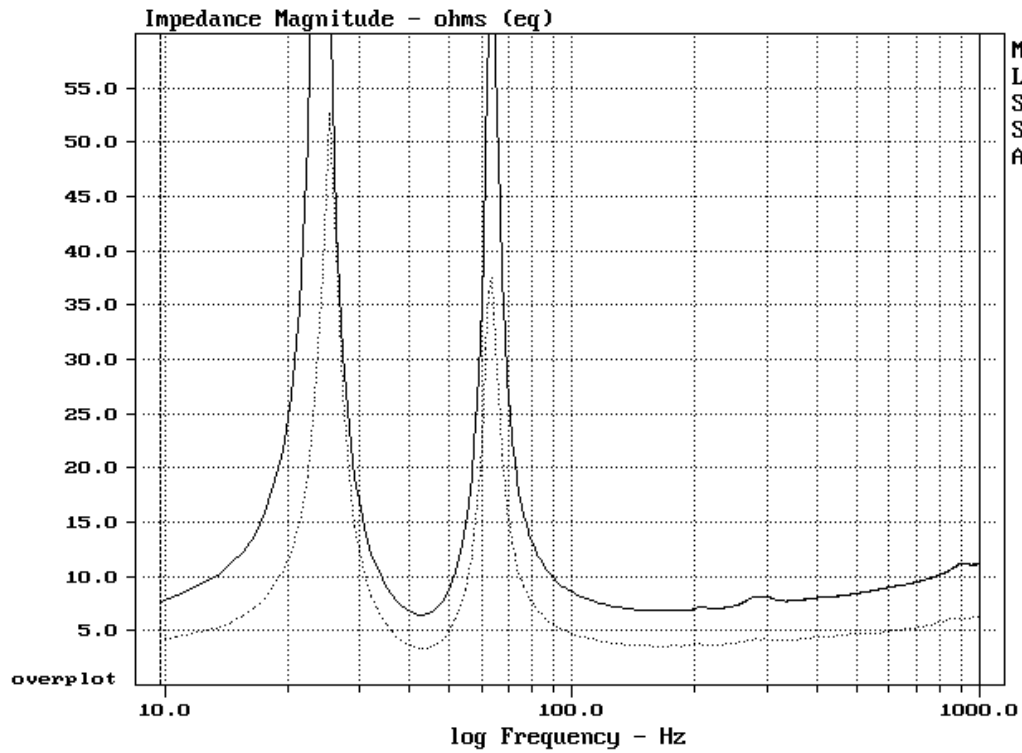
GAE BR15N Impedanzverlauf / Impedance Plot — 8Ω version minimum 6,5Ω @ 42Hz .... 4Ω version minimum 3,4Ω @ 42Hz
